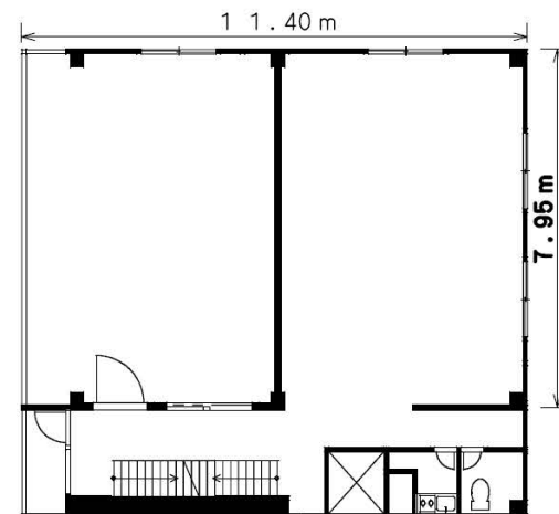
3階平面図 117.02㎡ (35.39坪)
