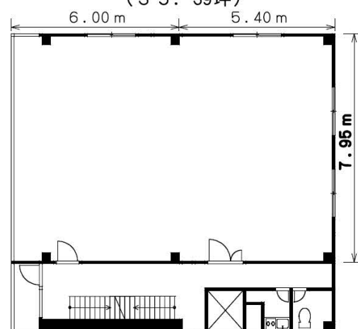
2階平面図 117.02㎡ (35.39坪)
